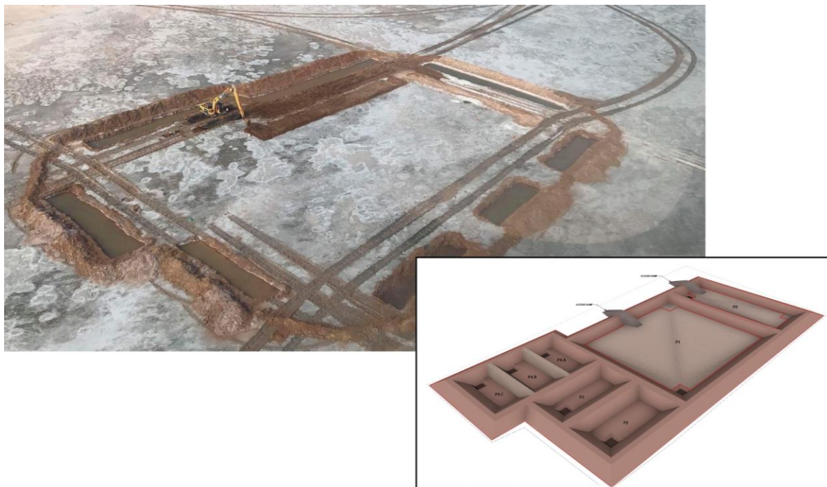
Figure 2. Pilot Evaporation Ponds Under Construction with 3D Schematic Design Inset
